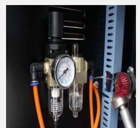
Adjustable Pressure
